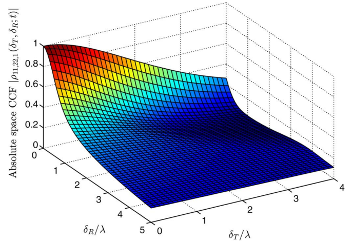
Fig. 6. Absolute space CCF |\rho_{11,22,1}(\delta_T, \delta_R; t)| of the ellipse model. ( M_R = M_T = 32 , t = 1 s, a_1 = 100 m, f = 80 m, D_c^a = 30 m, D_c^s = 50 m, \beta_R = \beta_T = \pi/2 , \lambda = 0.15 m, f_{\max} = 33.33 Hz, \alpha_v = \pi/6 , \kappa = 5 , NLOS).
