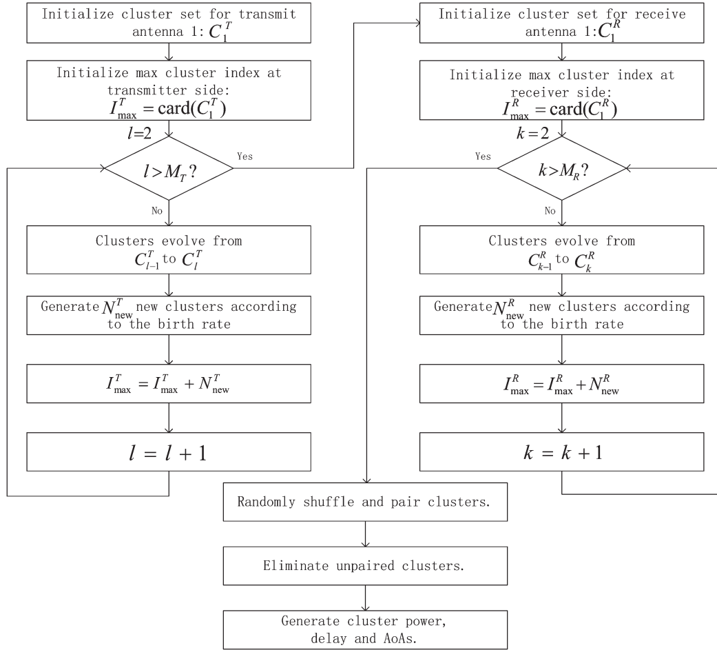
Fig. 2. Cluster generation algorithm flowchart.
