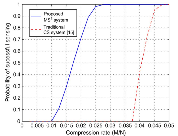
Fig. 6. Comparison between MS^3 and CS-based system [15]. The probability of successful sensing that is defined as the probability of achieving both P_d \geq 90\% and P_f \leq 10\% . In simulations, the average SNR as received at CRs is 10 dB, and the number of CRs is v = 22 .
