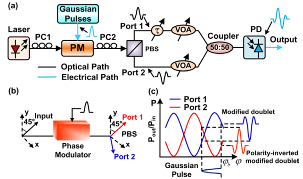
Fig. 1. (a) Schematic diagram of the proposal for power-efficient UWB pulse generation (b) illustration of modified doublets generator based on polarization interference (c) principle of shaping a Gaussian pulse into two complementary modified doublets.
